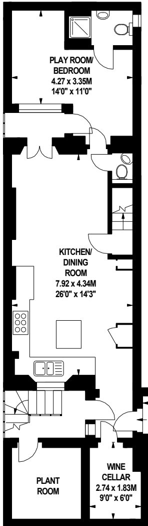
842 sq ft Lower Ground Floor
